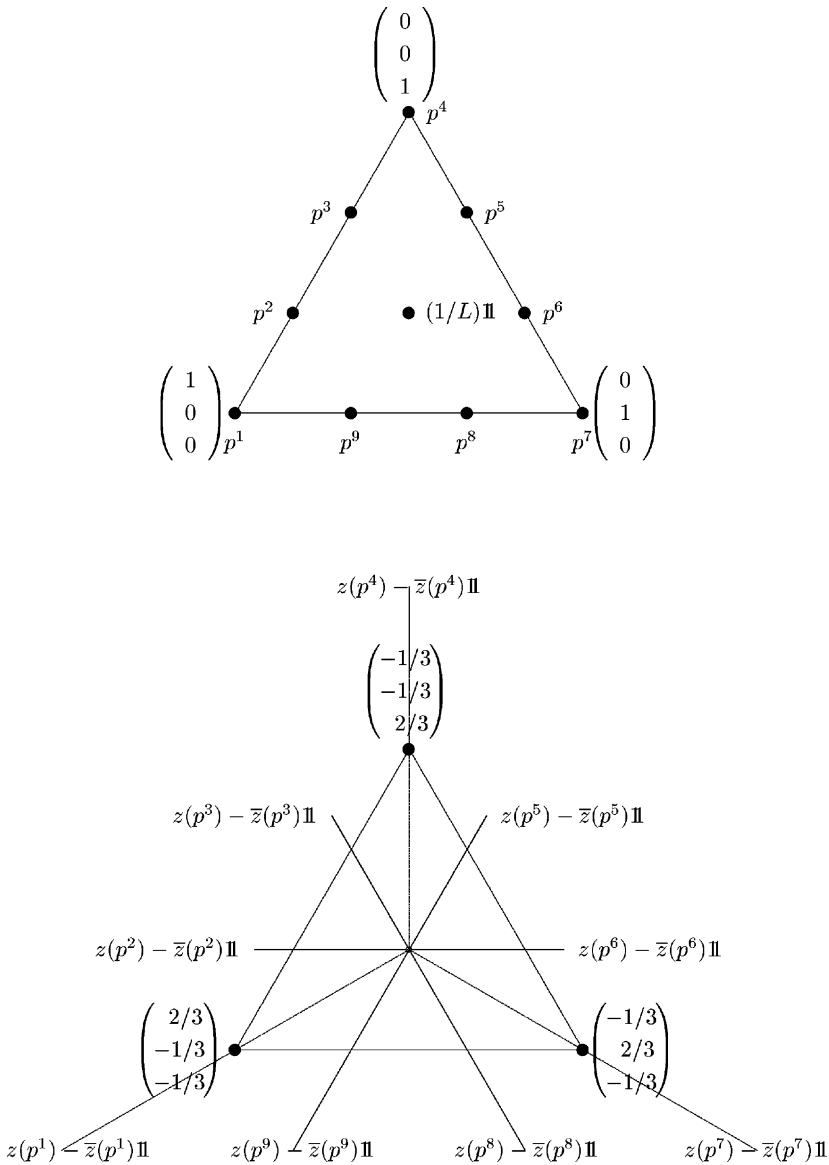
Fig. 3. A vector z(p) - \bar{z}(p)\mathbb{1} that is radially outward pointing for p = p^1, p^2, \dots, p^9 .
