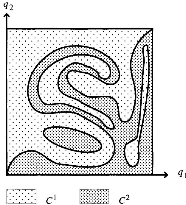
Fig. 1. Illustration of Theorem 3.1, case n=2 .
