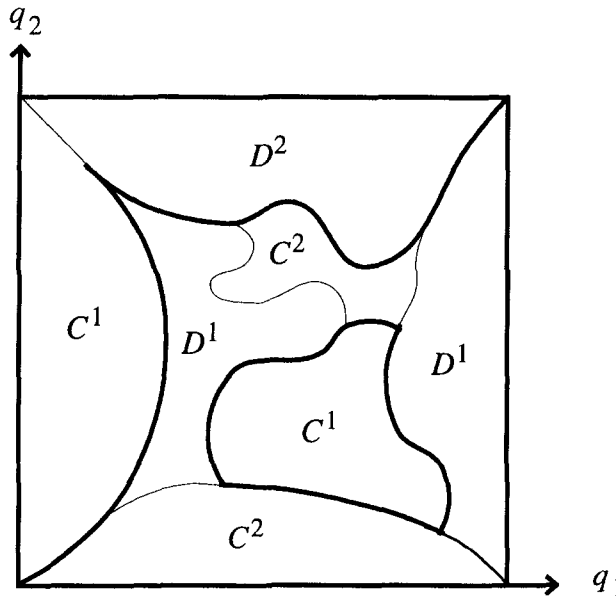
Fig. 2. Illustration of Theorem 3.4, case n=2 .
