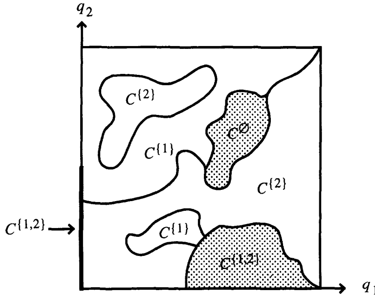
Fig. 3. Illustration of Theorem 3.6, case n=2 .
