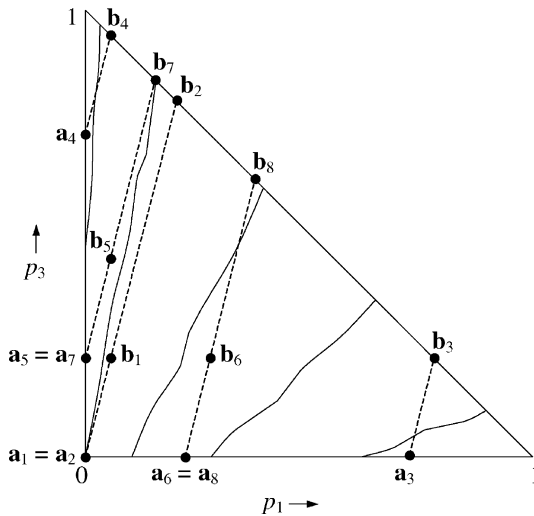
Fig. 2. Fanning-out.
