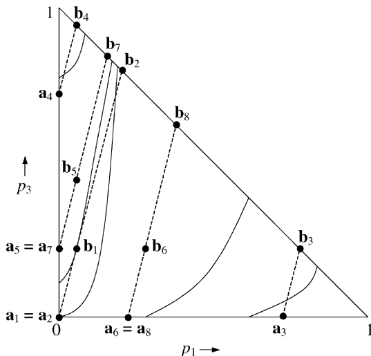
Fig. 3. Quasi-concavity.
